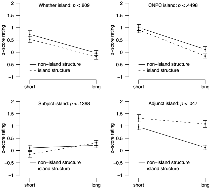
Figure 5. Island effects with Japanese single wh -questions. The p -values of the interaction term appear at the top.
