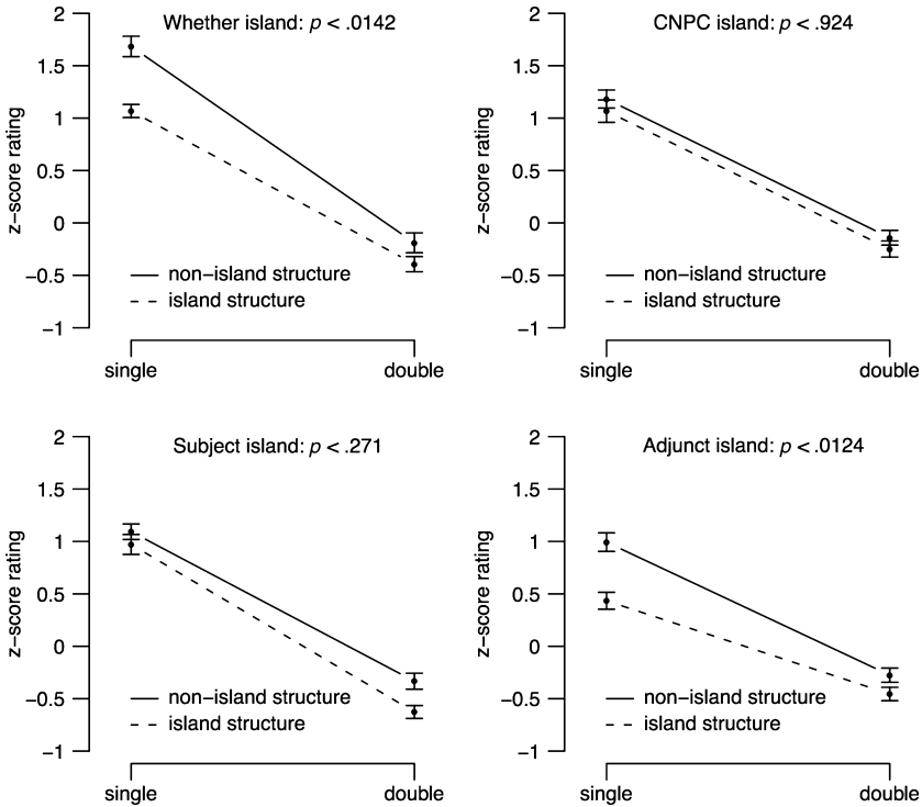
Figure 3. Island effects with English multiple wh -questions. The p -values of the interaction term appear at the top.
