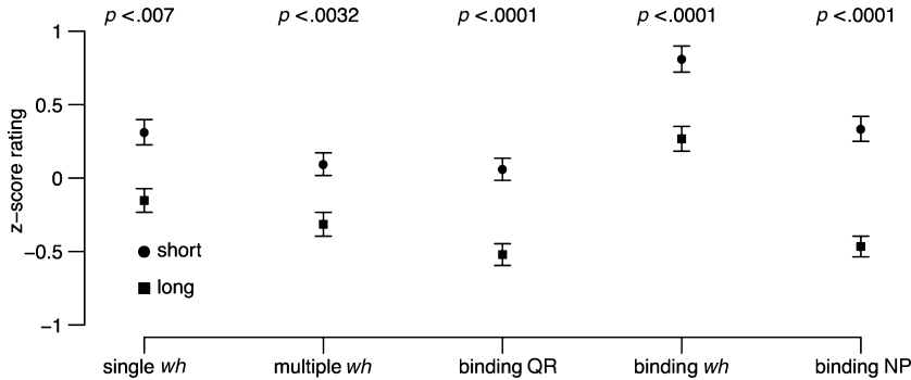
Figure 4. Length effects for constructions requiring search processes in English
