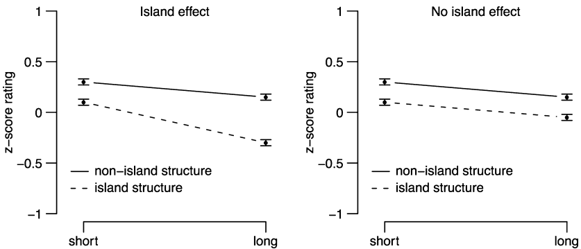
Figure 1. The potential results of the factorial definition of island effects
